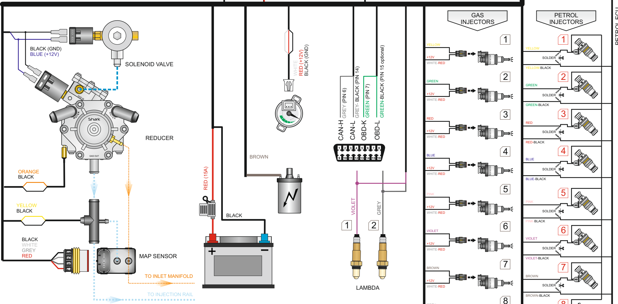
CONNECTION DIAGRAM OF THE LPG/CNG OPTIMA PRO-TEC INSTALLATION
