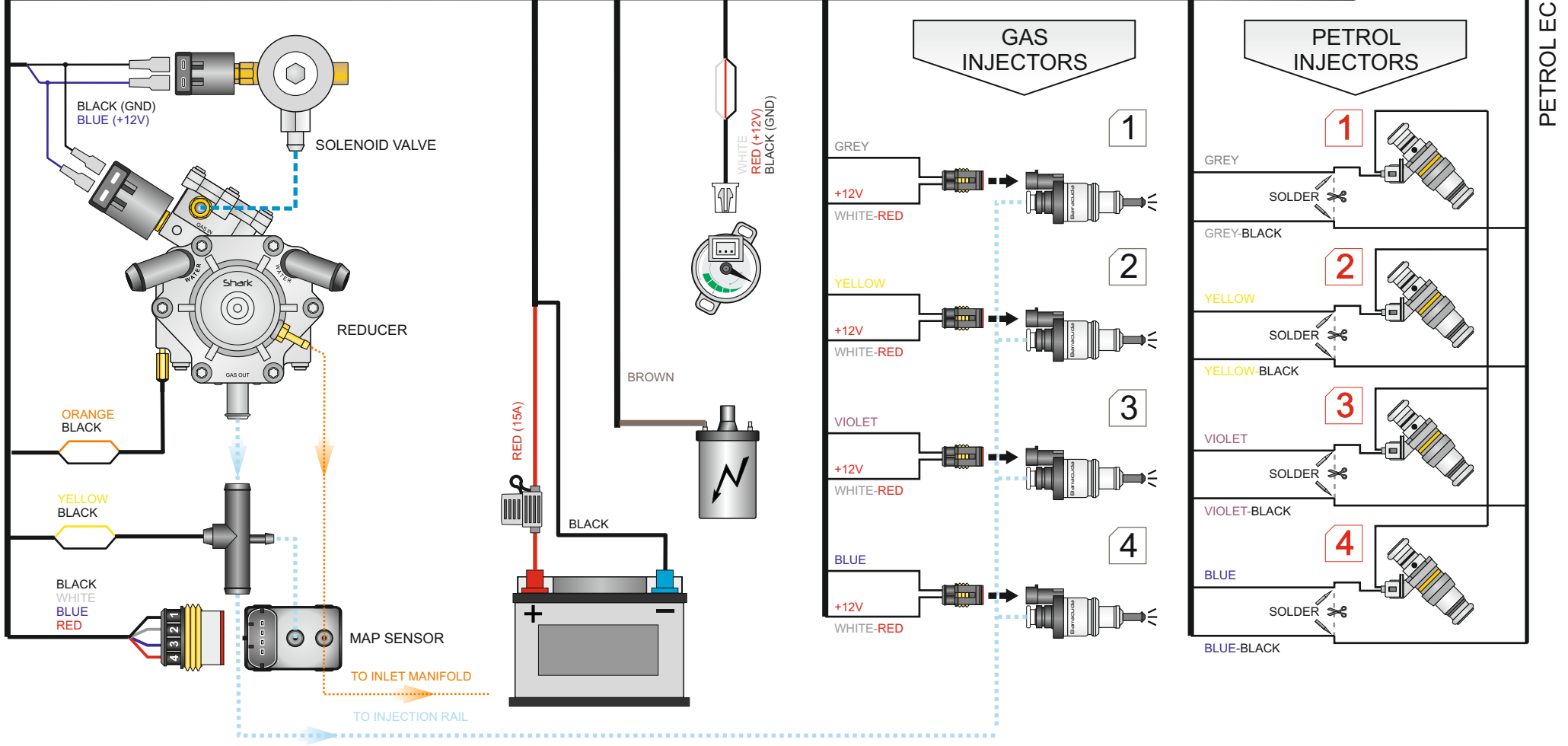
CONNECTION DIAGRAM OF THE LPG/CNG OPTIMA ECO-TEC INSTALLATION
